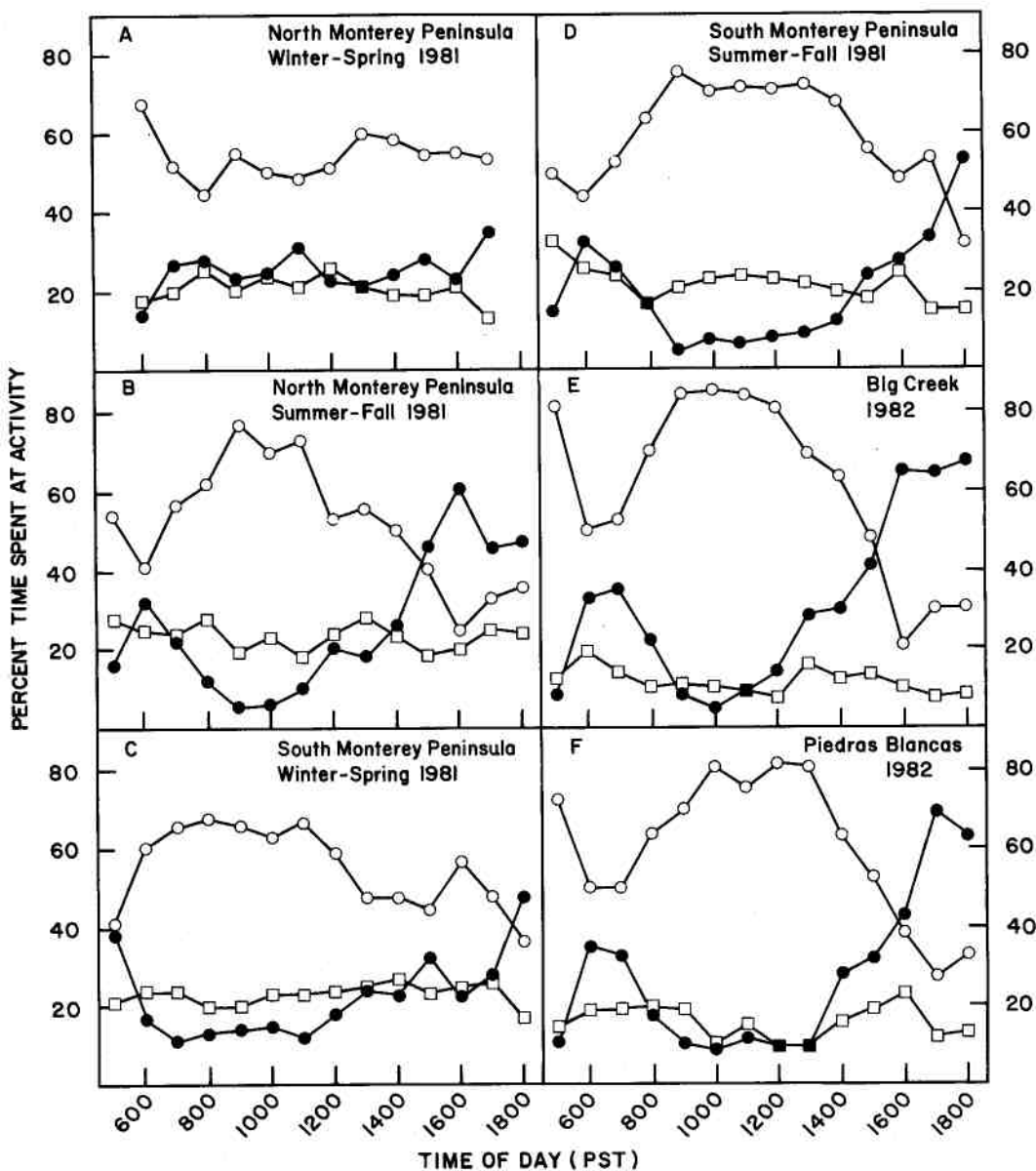
Fig. 2. Temporal patterns of sea otter activity at each of the 4 study areas in central California. Open circles = resting, closed circles = foraging, squares = other. (Dates were as follows: NMP winter-spring = Jan, Mar, and May; NMP summer-fall = Jul and Sep; SMP winter-spring = Feb and Apr; SMP summer-fall = Jun, Aug, and Oct; and BC and PB = Apr-Jul).
